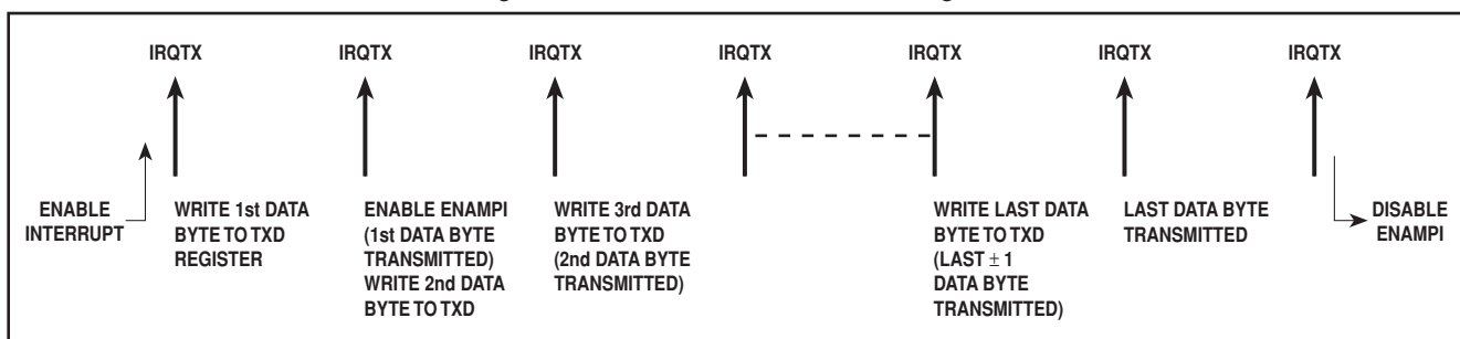
Figure 23 - Modem transmission sequence
